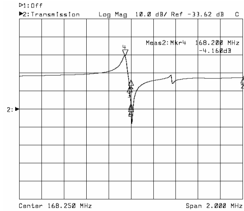
Horizontal: 0.2MHz/Div Vertical: 10dB/Div
